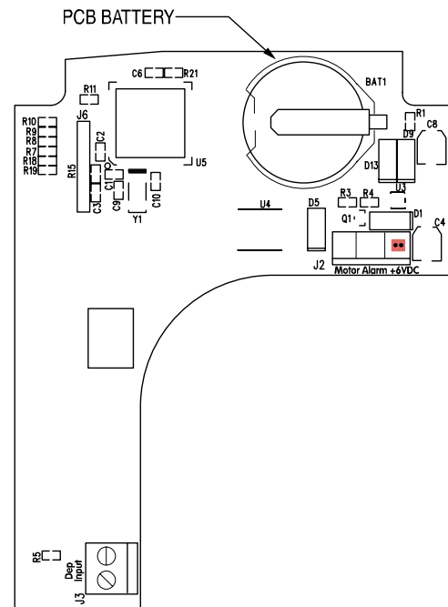
Figure 8.1. PoolShot Main PCB
