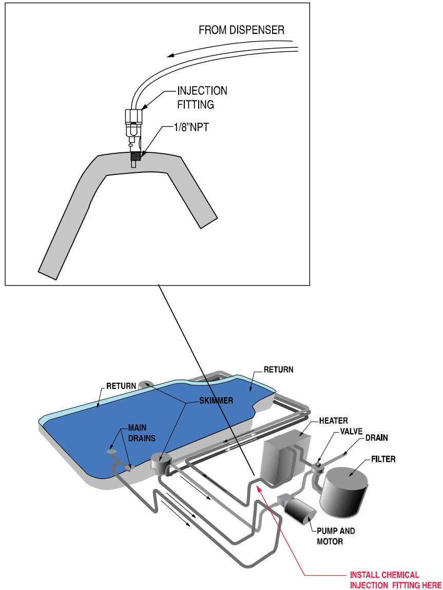
Figure 2. PoolShot Full Installation
