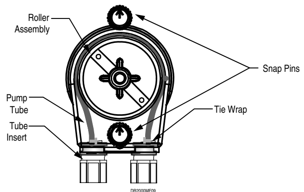
Figure 1b. SnapHead Pump Cartridge
